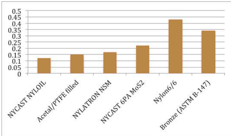
Chart 1: comparison coefficient of friction different materials, measured on thrust washer testing machine, unlubricated @ 40 fpm and 50 lb/iñ
